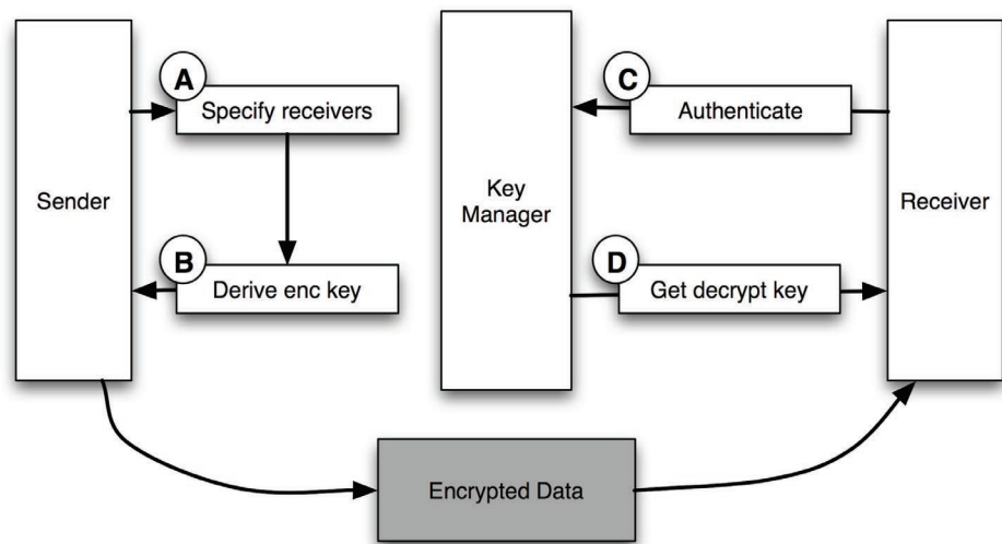
Figure 3: IBE diagram
